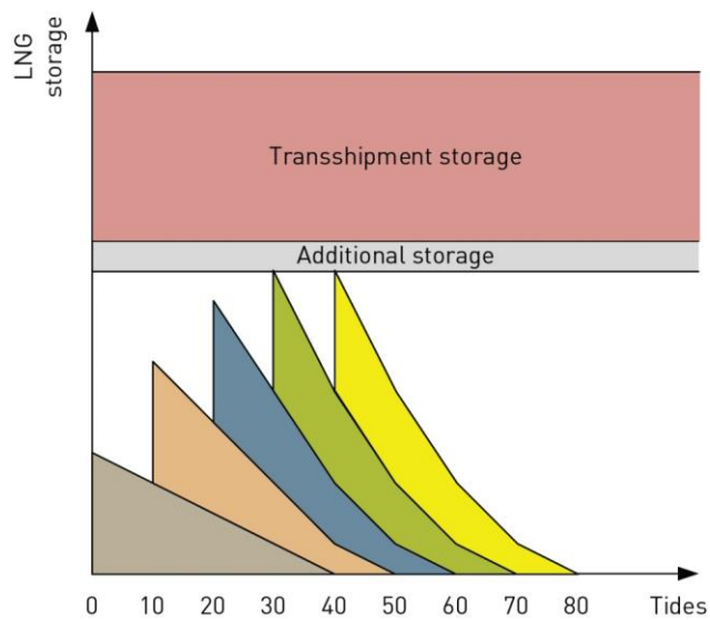
Figure 3.2 Storage capacity
