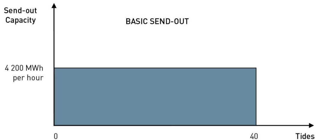
Figure 4.2 Basic send-out
