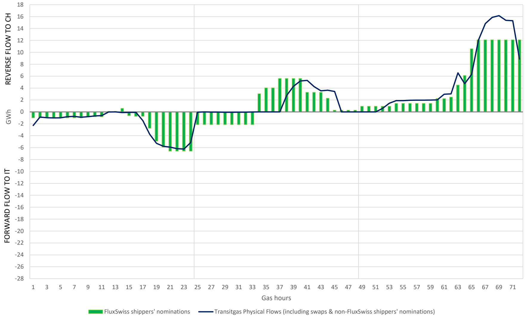
Passo Gries - Gas Days Friday 01/10/21 to Sunday 03/10/21 (>0 = entry into CH; <0 = exit from CH)
